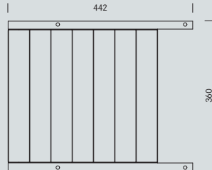
Maßskizze 5 Dimensional drawing 5
