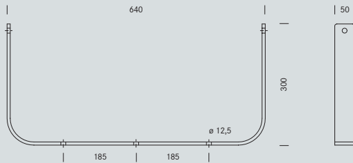
Maßskizze 3 Dimensional drawing 3
